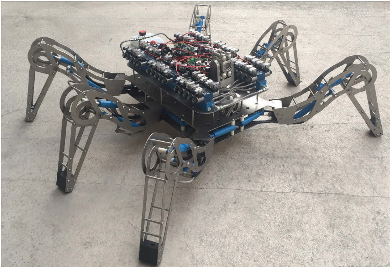
A spider-like robot designed to handle radioactive waste, Latro will be able to walk over and around obstacles.
